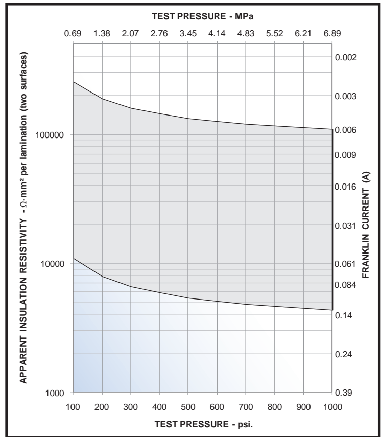
FIGURE 1 – TYPICAL SURFACE INSULATION CHARACTERISTICS
