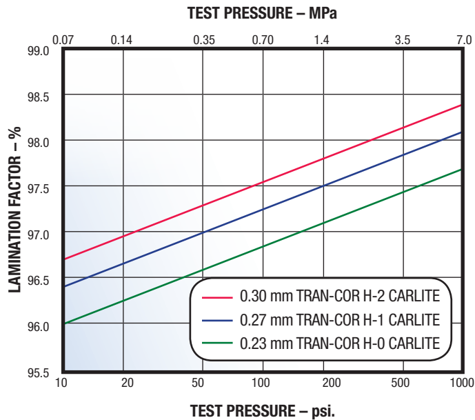
FIGURE 2 – REPRESENTATIVE LAMINATION FACTORS
